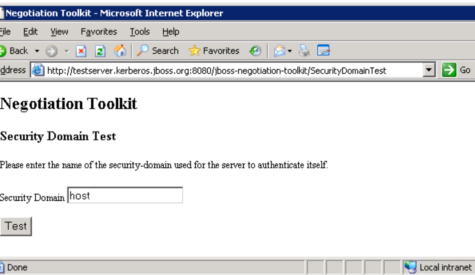
Figure 2.4. Security Domain Test
