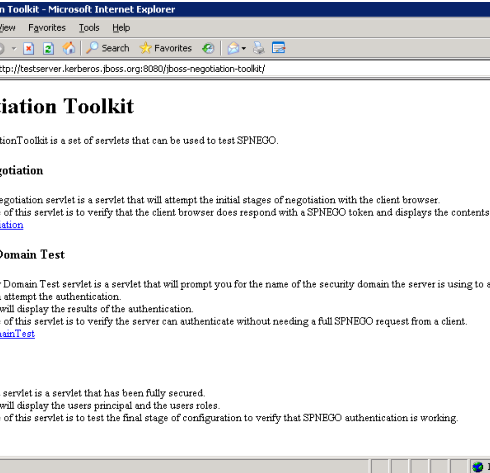
Figure 2.1. Negotiation Toolkit Front Page
