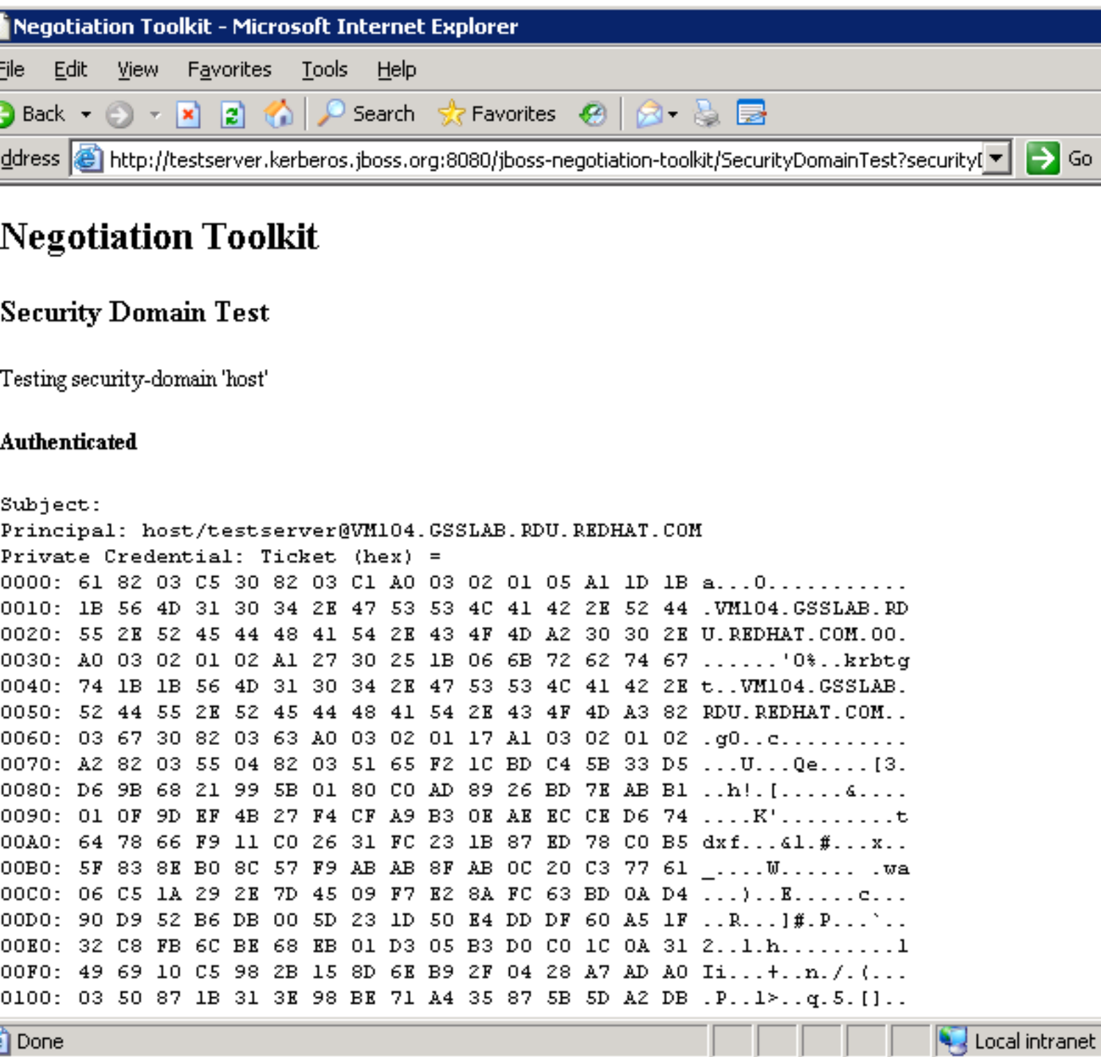
Figure 2.5. Security Domain Test - Authenticated
